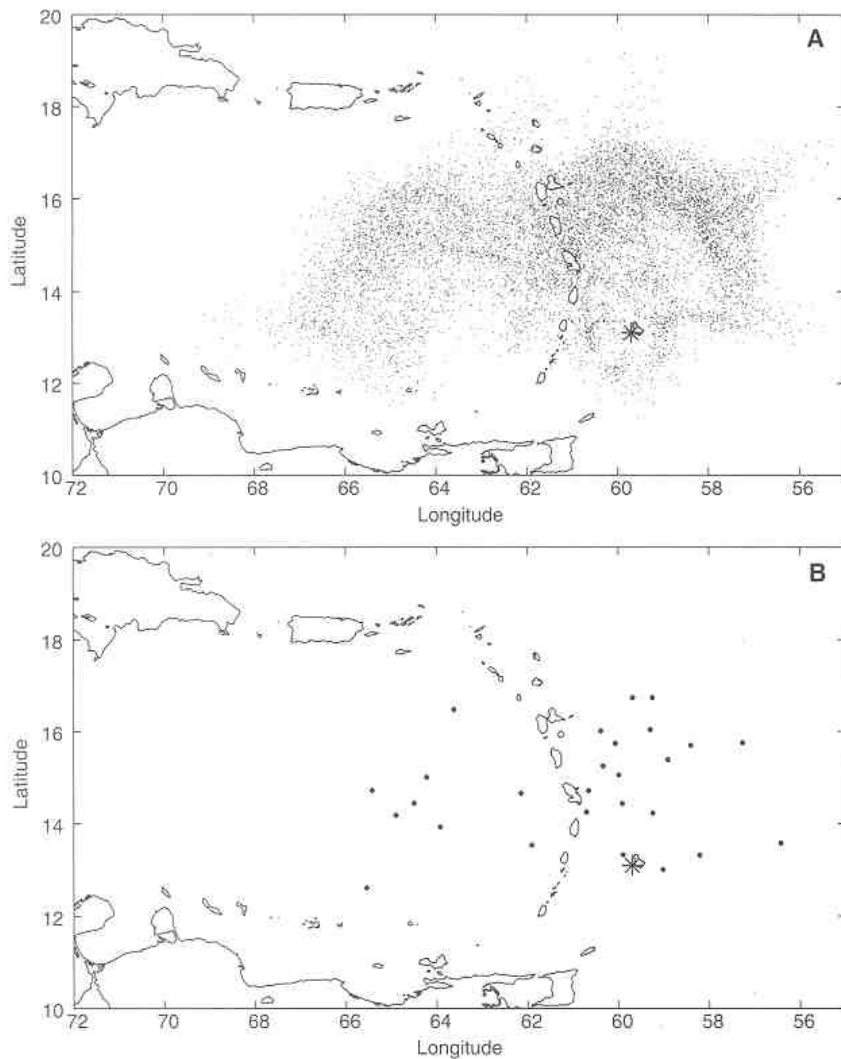
Fig. 2. Transport endpoints of 10,000 virtual larvae released from a 1-km 2 area off Barbados (*) using mixed layer flow model. (A) Model results of the dispersion of larvae after 30 days; (B) same model run as in (A) , but with effect of larval mortality at a typical rate of 18% day -1 ( \mu = 0.2 ). We used the Miami Isopycnic Coordinate Ocean Model (MICOM) (23) to model the circulation for a 30-day period. Subgrid turbulent motion of each virtual larva was modeled using a random flight model (24) with K = 10 \text{ m}^2 \text{ s}^{-1} . The MICOM model resolves mesoscale turbulence, thereby providing more realistic estimates of diffusive motion than that incorporated in the 2D model above.
