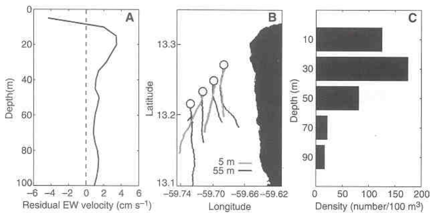
Fig. 3. Vertical structure of flow and larval fish distributions along the west coast of Barbados. (A) Onshore/offshore (east-west, indicated by E-W) component of residual flow at depths between 0 and 100 m; (B) GPS drifter tracks during one 12-hour experiment of Lagrangian flow along the west coast of Barbados; (C) Vertical distribution of postflexion larvae of the family Pomacentridae in each of five, 20 m depth bins to a maximum depth of 100 m. Residual flow was determined from ship-mounted, bottom-tracked 150-kHz ADCP during a 30-day cruise in May 1996. All current estimates were from a sampling domain extending 10 km offshore and 20 km along the western shore; we averaged by depth for the full 30-day period. Drifter tracks were determined from satellite-tracked, GPS drifters drogued with 1 \times 10 m holeysock drogues centered at 5 and 55 m. Each track represents approximately 8 to 12 hours of drift time. Point of deployment is denoted by open circle (○). Vertical distribution of larvae was determined from vertically discrete ichthyoplankton collections ( n = 176 stations) using a 1\text{-m}^2 MOCNESS, fitted with 333\text{-}\mu\text{m} mesh nets towed at 5 discrete depths: 0 to 20, 20 to 40, 40 to 60, 60 to 80, and 80 to 100 m.
